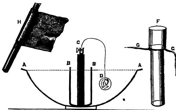
Fig. 171. A A. Basin containing the solution of sulphate of copper. B B. The porous cell, containing dilute sulphuric acid. C. Amalgamated zinc rod and binding screw attached to wire and medal D. F. Porous cell, made with a lamp-glass closed at small end by bladder and wire support G G, to prevent the membrane touching the bottom of the pan containing the solution of sulphate of copper. H. Brown paper porous cell, prepared by rolling paper of the required length at least three times round a ruler, and closing the sides and bottom with sealing-wax after the bottom is folded in.
